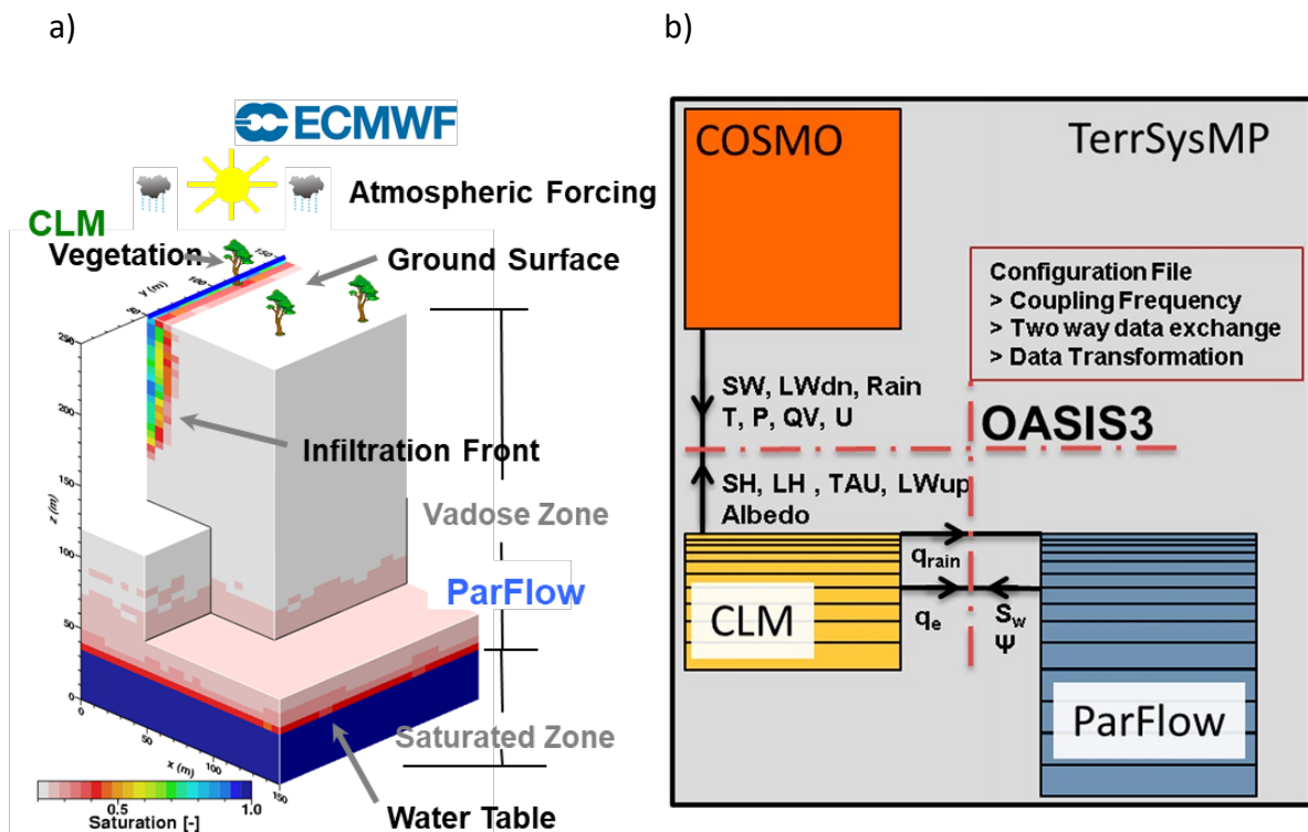
Figure 2: (a) The Terrestrial System Modeling Platform (TSMP) combines the compartment models COSMO, CLM and ParFlow. (b) The exchange of information about fluxes and states occurs at the conceptual boundaries (Shrestha et al., 2014).
